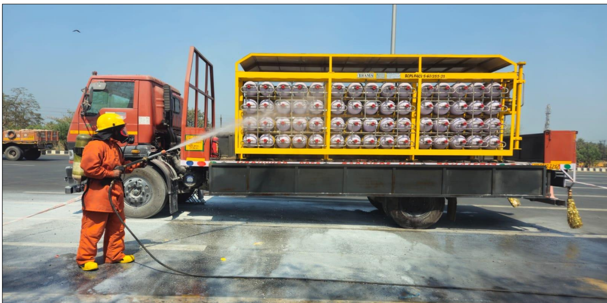
2. Fire Fighting by BGCL QRV Crew
